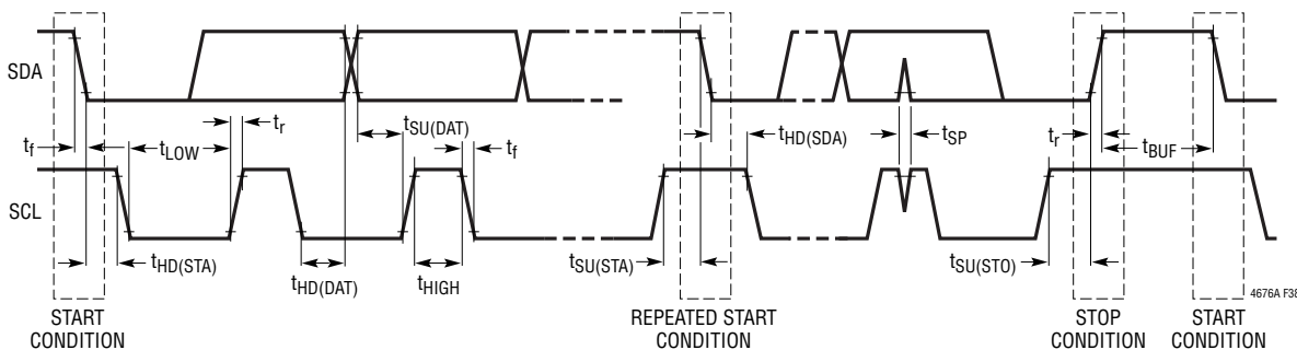
Figure 44. Timing Diagram
