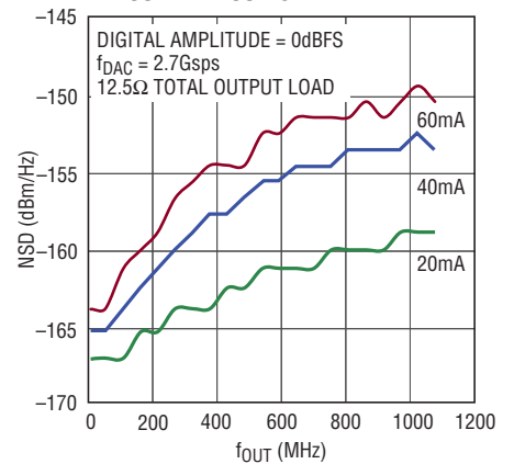
LTC2000A-16 Single-Tone NSD vs f_{OUT} and I_{OUTFS}
