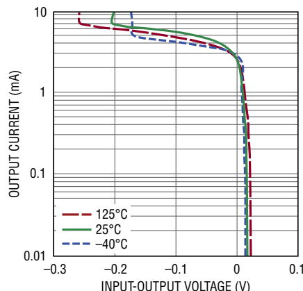
5V Minimum V IN -V OUT Differential (Sinking)
