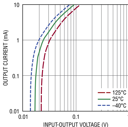
5V Minimum V IN -V OUT Differential (Sourcing)
