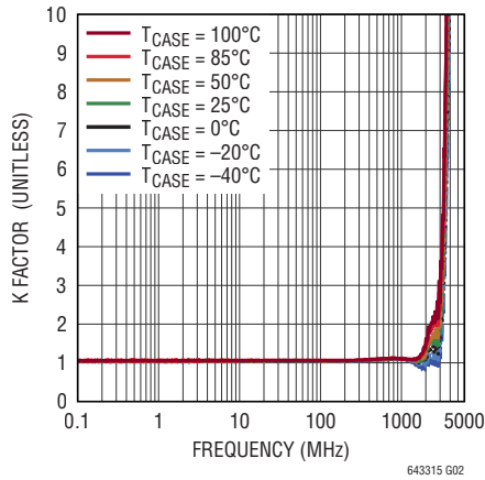
K Factor vs Frequency Over Temperature
