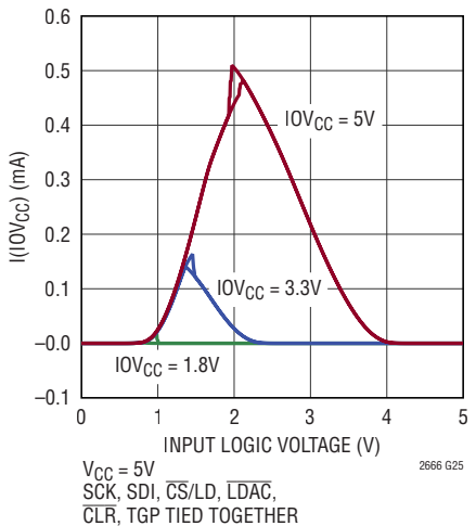
IOV_{CC} Supply Current vs Logic Voltage
