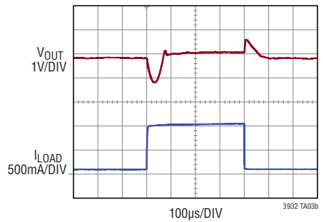
Load Step Response (100mA to 1A)
