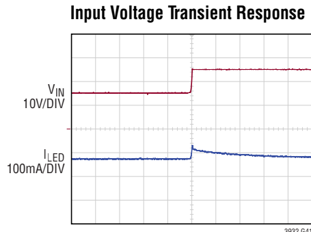
FRONT PAGE APPLICATION 15V TO 25V INPUT VOLTAGE STEP 3 LEDs (APPROX. 9V)
