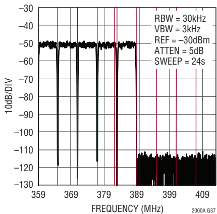
32-Carrier DOCSIS Low Band Narrowband ACLR, f_{DAC} = 2.7Gps
