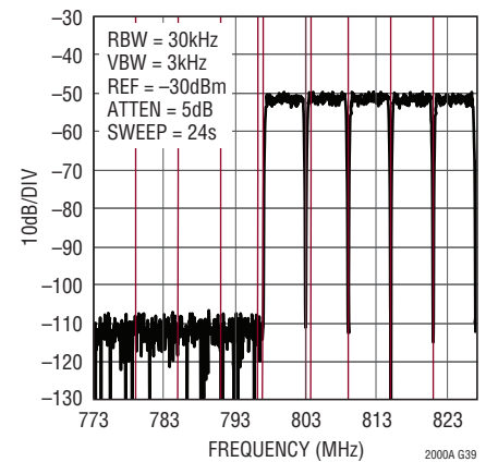
32 Carrier DOCSIS High Band Narrowband ACLR, f_{DAC} = 2.7Gps
