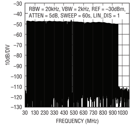
157 Carrier Tones with Gap Channel Wideband ACLR, f_{DAC} = 2.7Gsp/s
