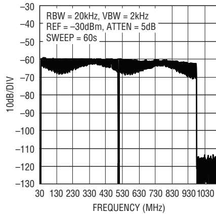
157 Carrier DOCSIS Gap Channel Wideband ACLR, f_{DAC} = 2.7Gsp/s
