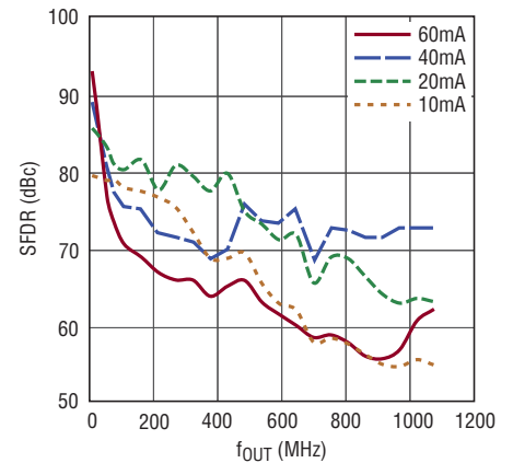
SFDR vs f_{OUT} and I_{OUTFS} , f_{DAC} = 2.7Gsp/s
