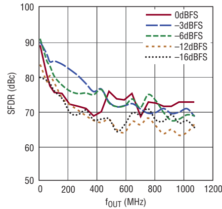
SFDR vs f_{OUT} and Digital Amplitude (dBFS), f_{DAC} = 2.7Gsp/s
