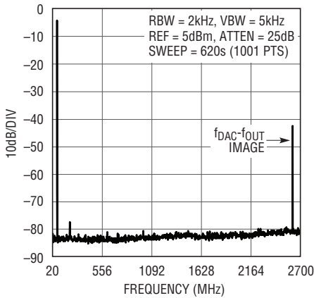
Single-Tone Spectrum at f_{OUT} = 70MHz , f_{DAC} = 2.7Gsp/s
