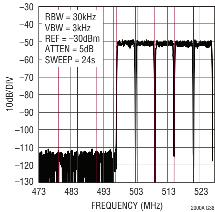
32 Carrier DOCSIS Mid Band Narrowband ACLR, f_{DAC} = 2.7Gps
