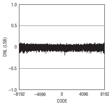
LTC2000A-14 Differential Nonlinearity (DNL)
