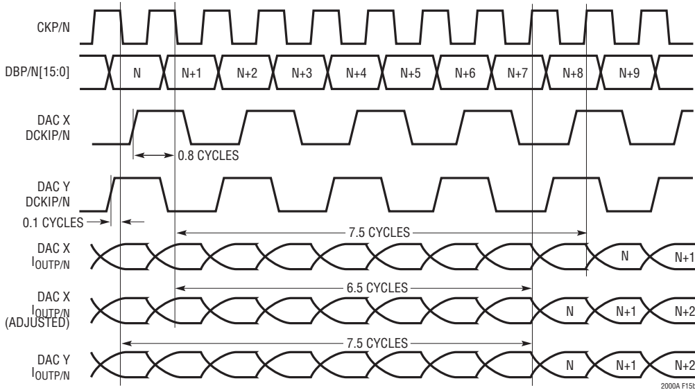
Figure 15b. Sample Waveforms — Synchronizing Multiple LTC2000As in Single Port Mode
