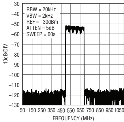
32-Carrier DOCSIS Mid Band Wideband ACLR, f_{DAC} = 2.7Gps
