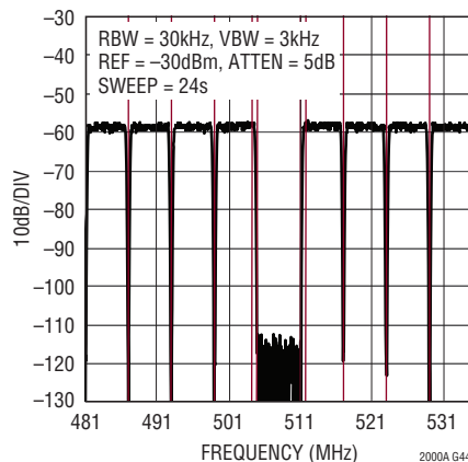
157 Carrier DOCSIS Gap Channel Narrowband ACLR, f_{DAC} = 2.7Gsp/s
