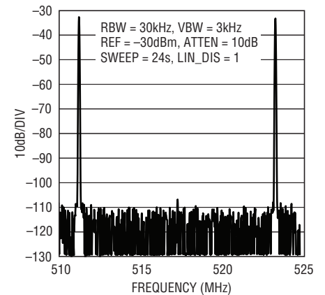
157 Carrier Tones with Gap Channel Narrowband ACLR, f_{DAC} = 2.7Gsp/s
