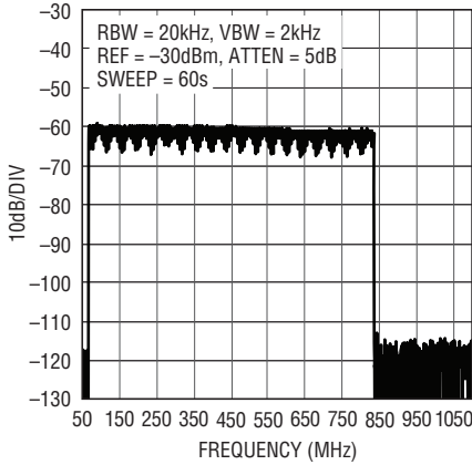
128 Carrier DOCSIS Low Band Wideband ACLR, f_{DAC} = 2.7Gsp/s
