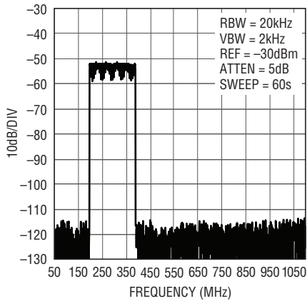
32-Carrier DOCSIS Low Band Wideband ACLR, f_{DAC} = 2.7Gps
