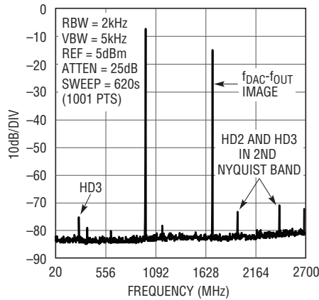
Single-Tone Spectrum at f_{OUT} = 990MHz , f_{DAC} = 2.7Gsp/s
