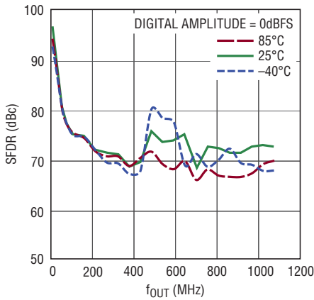
SFDR vs f_{OUT} and Temperature, f_{DAC} = 2.7Gsp/s
