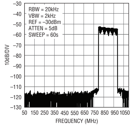
32 Carrier DOCSIS High Band Wideband ACLR, f_{DAC} = 2.7Gps
