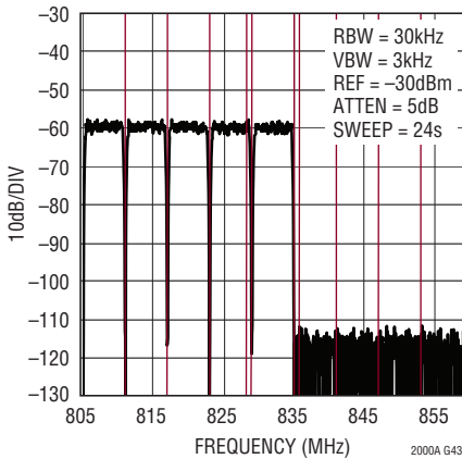
128 Carrier DOCSIS Low Band Narrowband ACLR, f_{DAC} = 2.7Gsp/s
