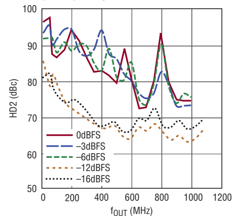
HD2 vs f_{OUT} and Digital Amplitude (dBFS), f_{DAC} = 2.7Gsp/s
