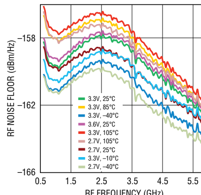
Noise Floor vs RF Frequency
