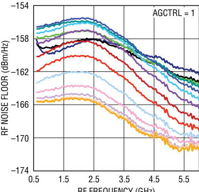
Noise Floor vs RF Frequency and V CTRL
