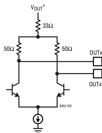
Figure 2. Simplified CML Interface Schematic (All OUTx)
