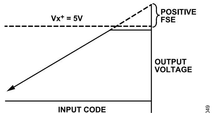
Figure 60. Effect of Negative Offset for Codes Near Zero Scale
