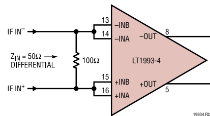
Figure 3. Alternate Input Termination for Differential 50\Omega Input Impedance
