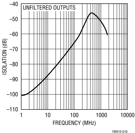
Reverse Isolation vs Frequency
