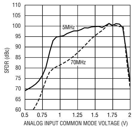
LTC2215 SFDR vs Analog Input Common Mode Voltage, 5MHz and 70MHz, -1\text{dBFS}
