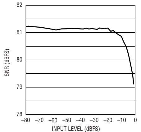
LTC2216 SNR vs Input Level, f_{IN} = 140.5\text{MHz}
