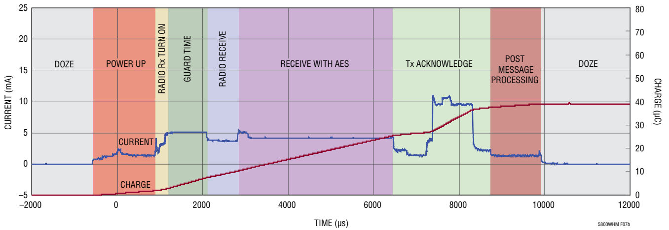
Atomic Operation – Maximum Length Transmit with Acknowledge, 10ms Time Slot (39.2µC Total Charge at 3.6V), 25°C, LTC5800I
