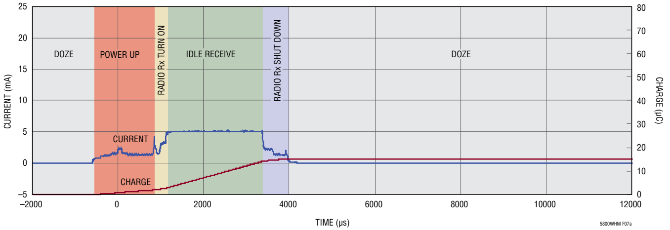
Atomic Operation – Idle Listen, 10ms Time Slot (15.1µC Total Charge at 3.6V), 25°C, LTC5800I
