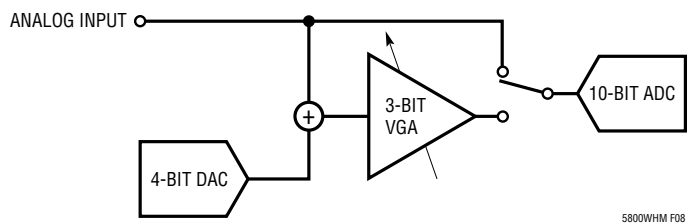
Figure 8. Analog Input Chain
