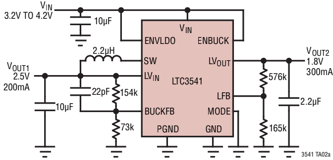
Dual Output with Minimal External Components Using Auto Start-Up Sequence, Buck in Burst Mode Operation for High Efficiency Down to Low Load Currents
