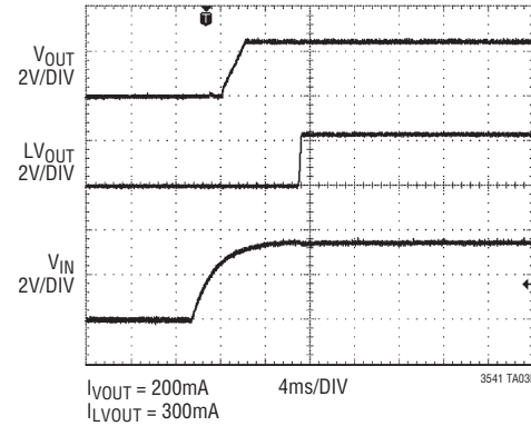
Dual Output with Minimal External Components Using Auto Start-Up Sequence, Buck in Pulse Skip Mode for Low Noise Operation
