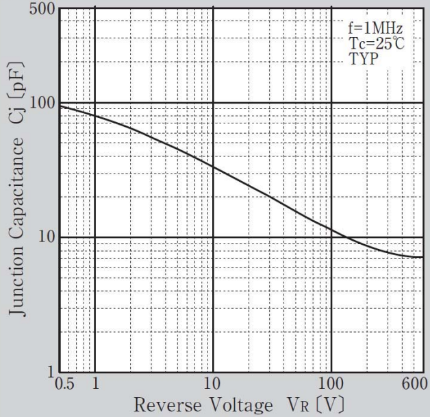
Junction Capacitance
