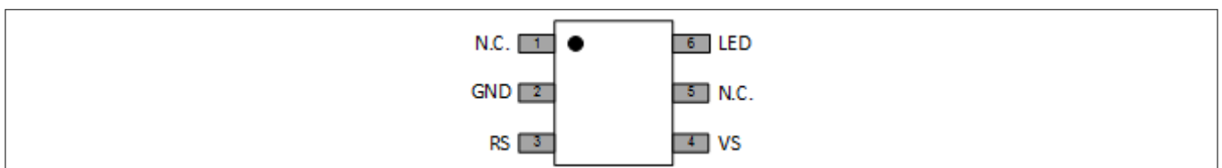
Figure 2 Pinout BCR431U
