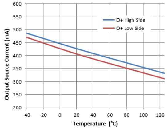
Figure 16. Output Source Current vs. Temperature
