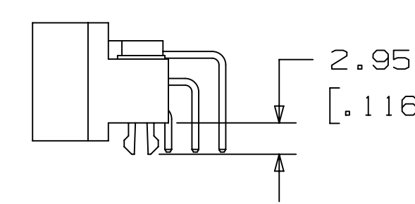
OPTIONAL RRIL WITH 'B' RETENTION CLIP (FOR .062 PCB THICKNESS)
