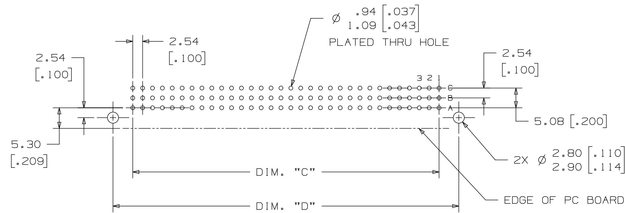
RECOMMENDED HOLE PATTERN (AS VIEWED FROM CONNECTOR SIDE)
