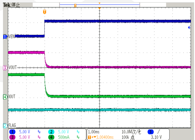
EN Turn Off (I load =0.7A, V in =5V, R=7ohm)
