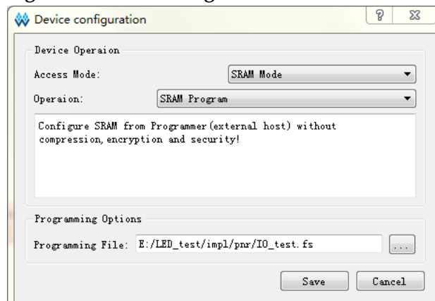
Figure 7 Device Configuration
