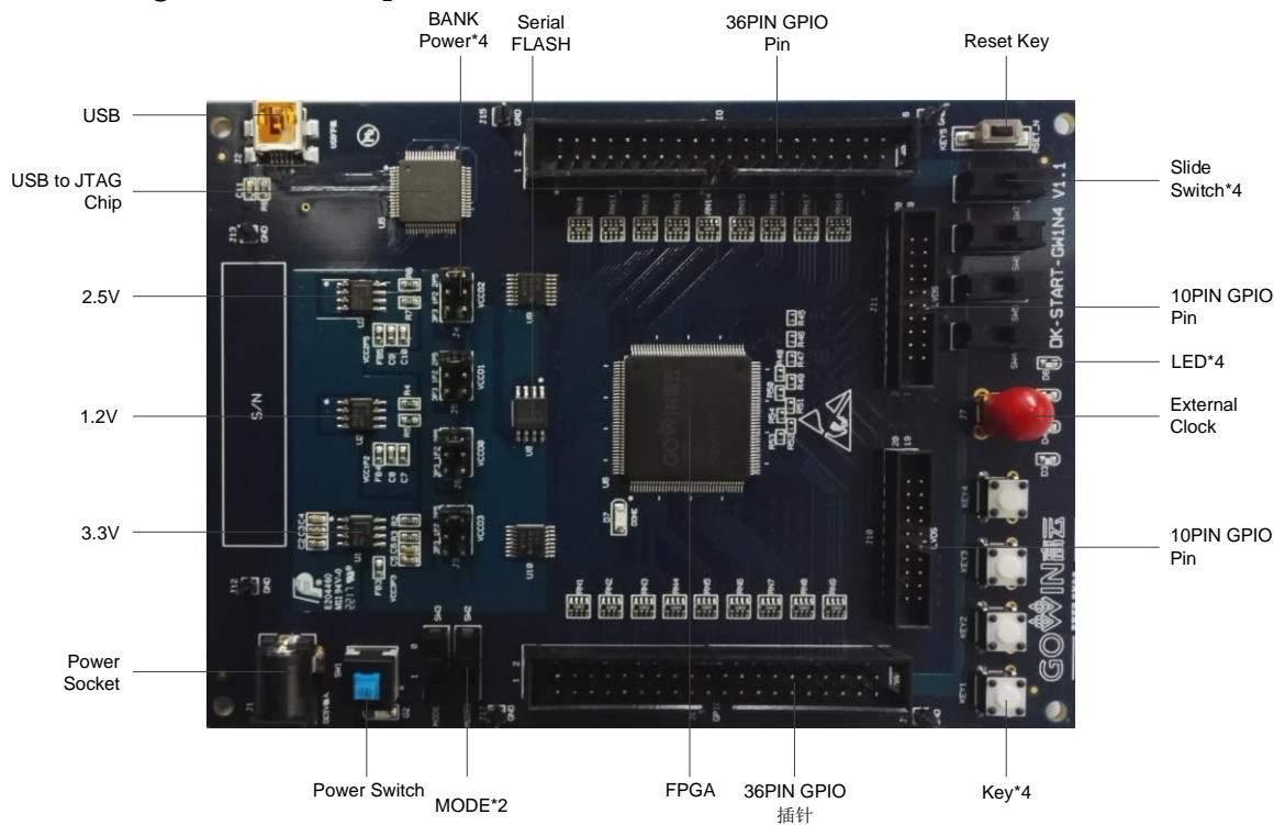
Figure 1 PCB Components
