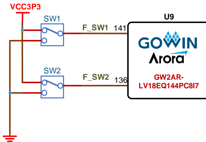
Figure 3-5 Switch Circuit
