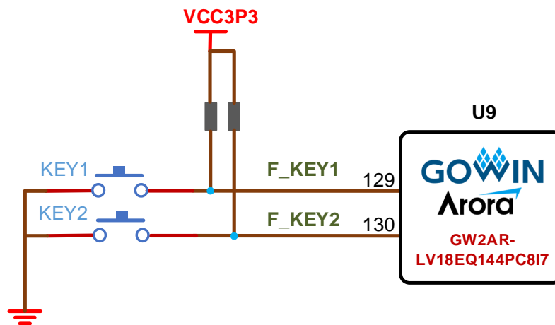
Figure 3-6 Key Circuit
