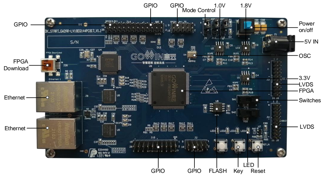
Figure 2-3 PCB Components
