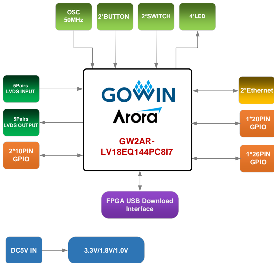
Figure 2-4 System Architecture
