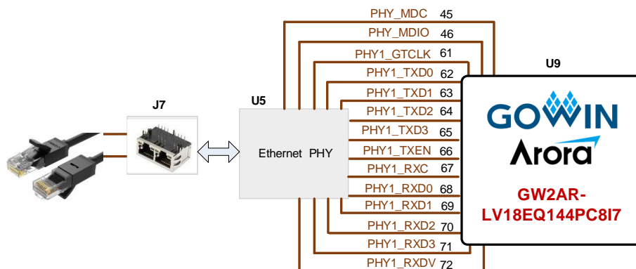
Figure 3-9 Ethernet Download Connection
