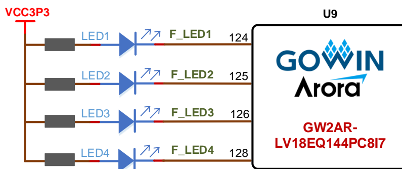
Figure 3-4 LED Circuit
