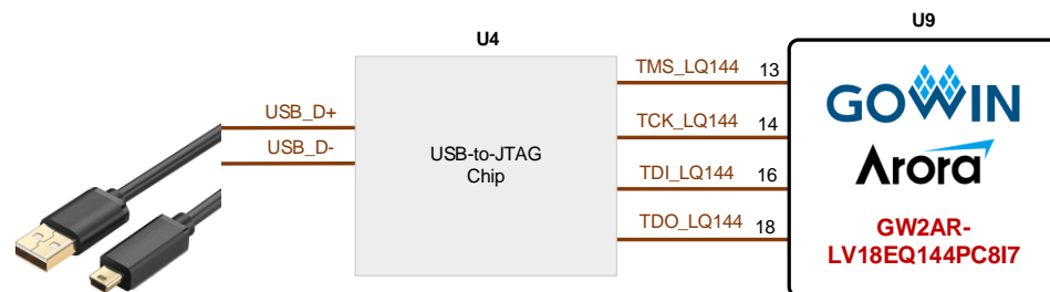
Figure 3-1 Connection Diagram for FPGA USB Downloading
