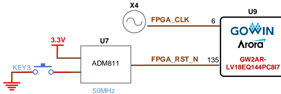
Figure 3-3 Clock, Reset
