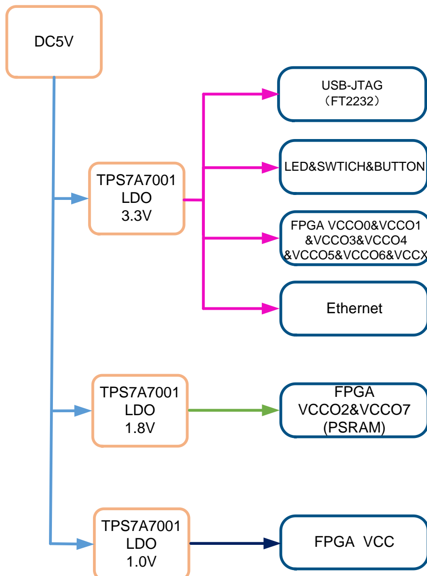
Figure 3-2 Power System Distribution
