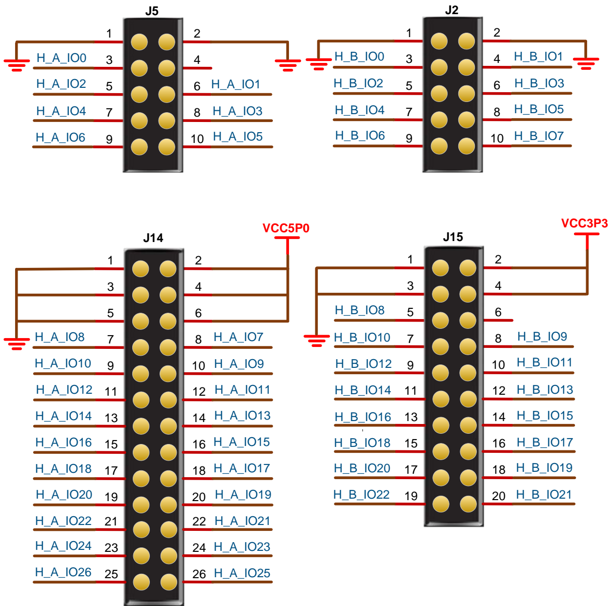
Figure 3-7 GPIO Circuit
