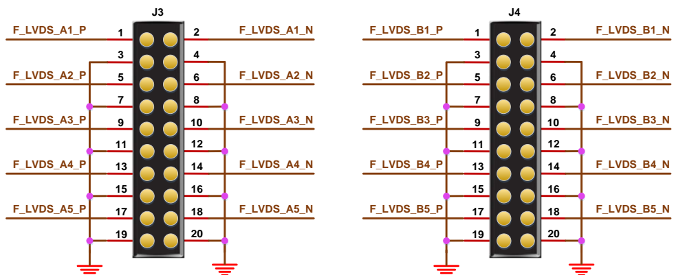
Figure 3-8 LVDS Circuit
