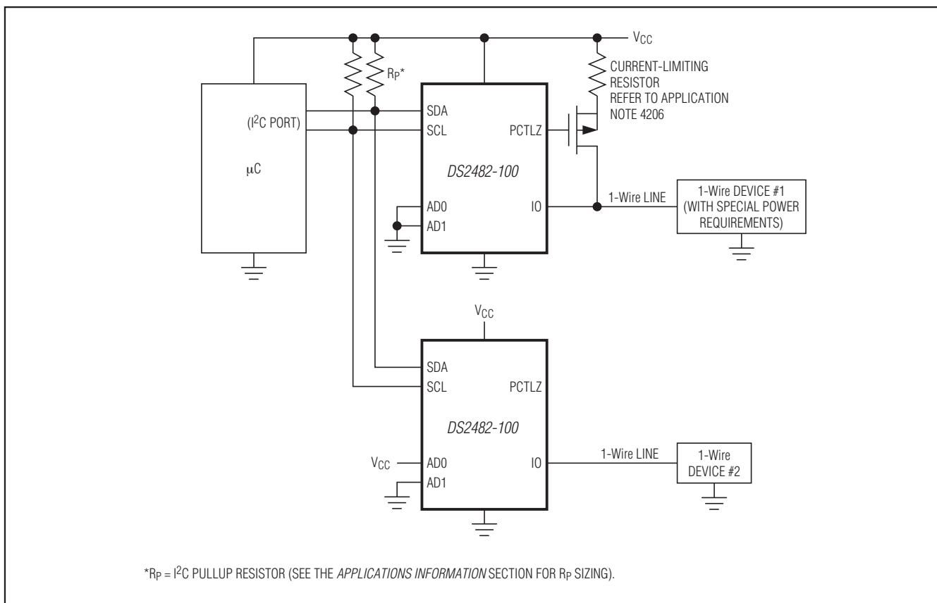
Figure 10. Application Schematic
