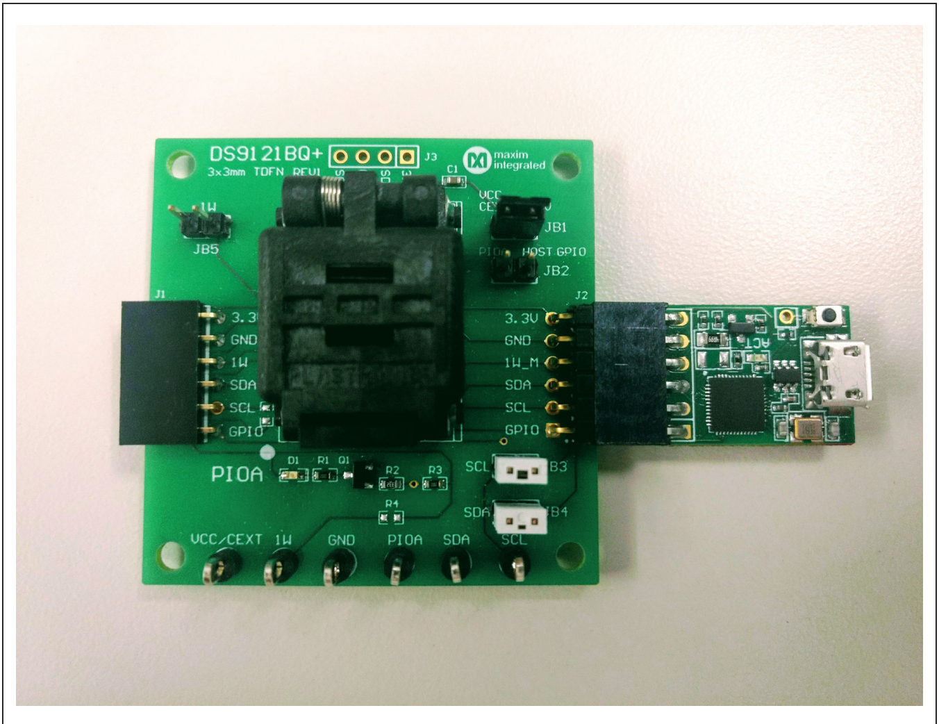
Figure 8. DS9481 Connected to DS28C50
