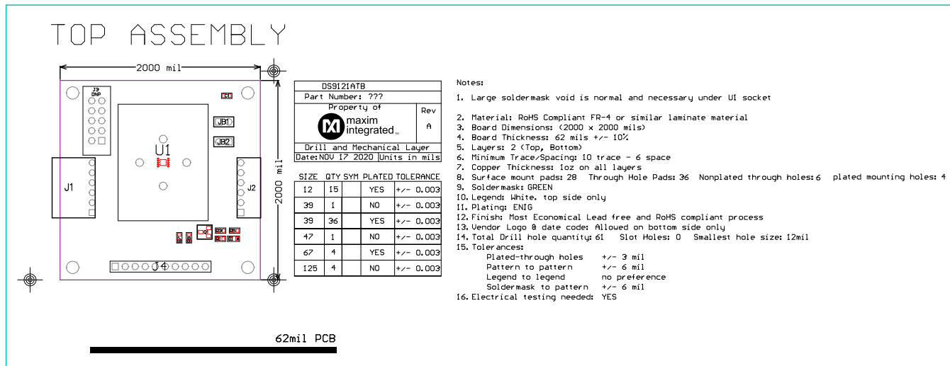
DS28E40 EV Kit PCB—Top Assembly
