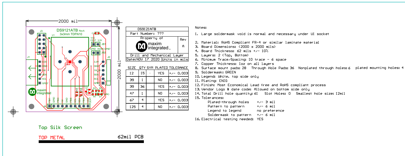
DS28E40 EV Kit PCB—Top Silkscreen
