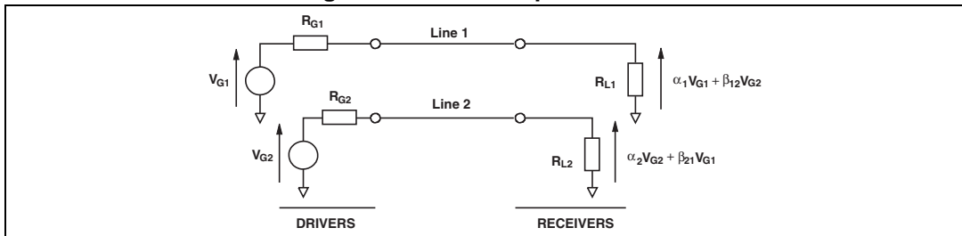
Figure 17. Crosstalk phenomena
