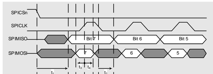
Figure 4: SPI Detailed Timing Diagram
