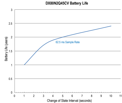
Figure 4. Battery Life
