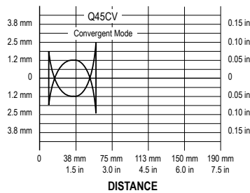
Figure 3. Beam Pattern
