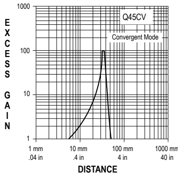
Figure 2. Excess Gain
