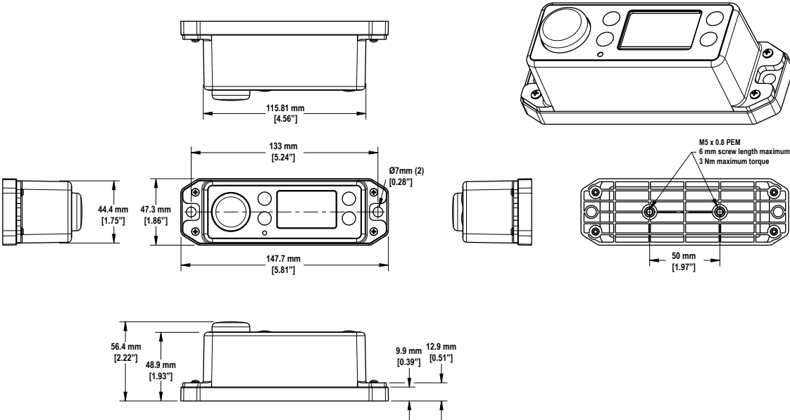
Figure 4. DSTS-QD dimensions
