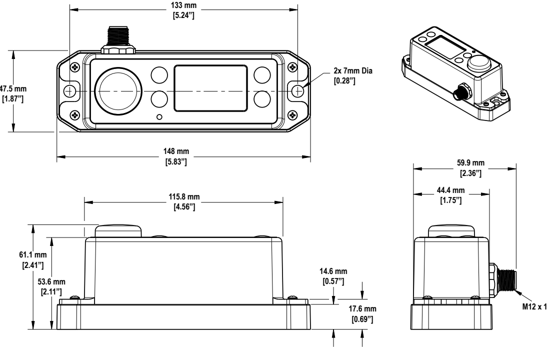
Figure 4. DSTS-QD dimensions
