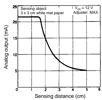
E32-DC200D/D4 with E3XA-CC4A analog amplifier
