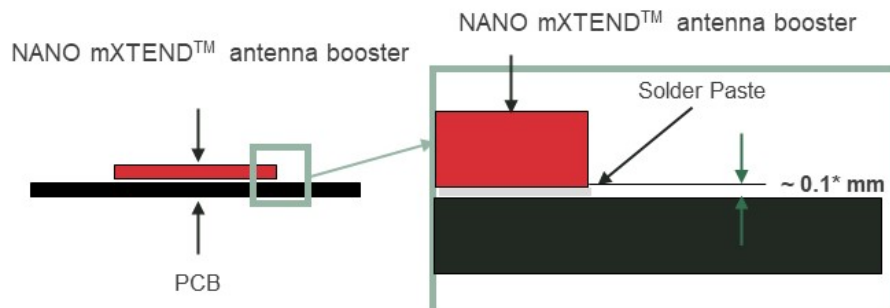
Figure 11 - Soldering details
