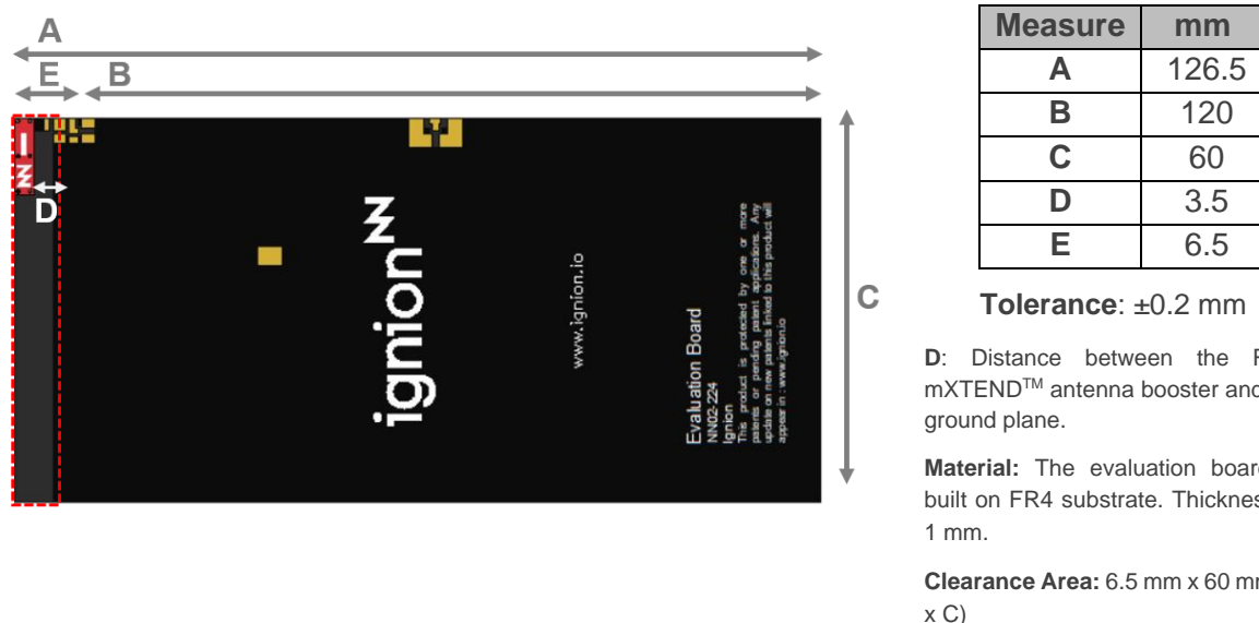
Figure 4 EB_NN02-224-1561-1606. Evaluation Board providing operation at BeiDou E1 band (1561 MHz), GPS L1 band (1575 MHz) and for GLONASS L1 band (from 1598 MHz to 1606 MHz).
