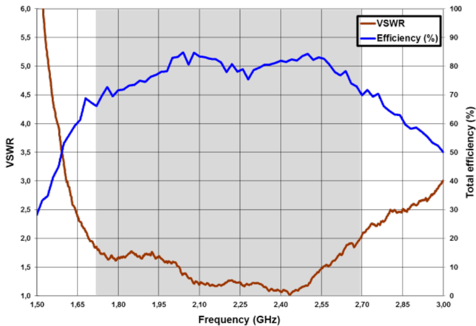
Figure 4 – VSWR and Total Efficiency for the 1710 – 2690 MHz range (from the Evaluation Board with UFL cables (Figure 1)).
