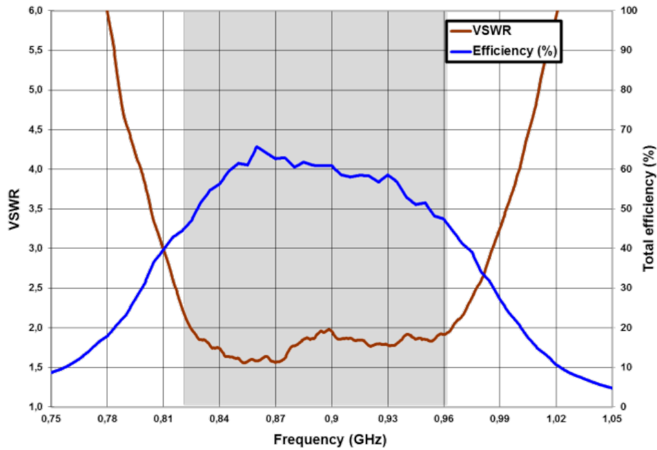
Figure 3 – VSWR and Total Efficiency for the 824 – 960 MHz range (from the Evaluation Board with UFL cables (Figure 1)).
