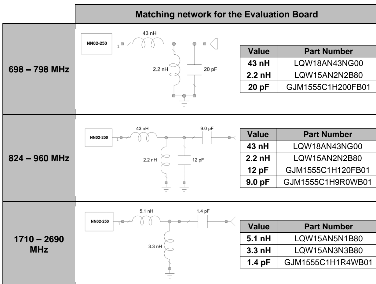
Figure 6 – Matching networks for the 3 ports solution (Evaluation Board with coplanar transmission lines).
