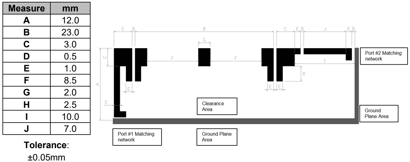
Figure 7 – Footprint dimensions for the single chip antenna component.
