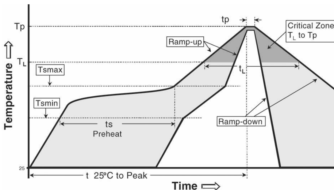
Figure 20 – Temperature profile.
