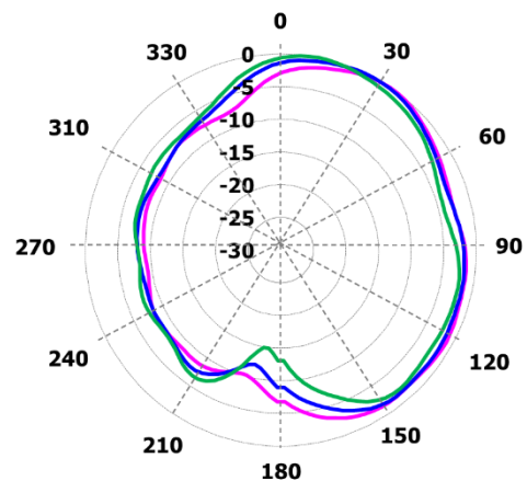
\phi = 90^\circ Plane YZ at 3.4 GHz, 3.6 GHz and 3.8 GHz
