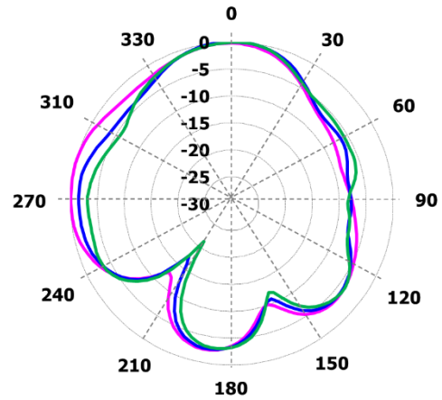
\theta = 90^\circ Plane XY at 3.4 GHz, 3.6 GHz and 3.8 GHz
