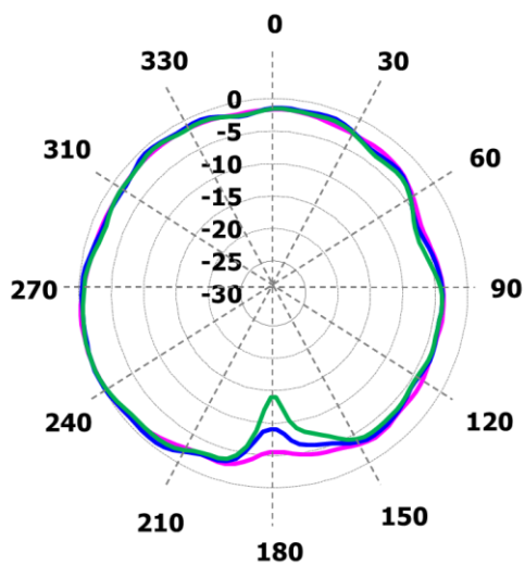
\phi = 0^\circ Plane XZ at 3.4 GHz, 3.6 GHz and 3.8 GHz
