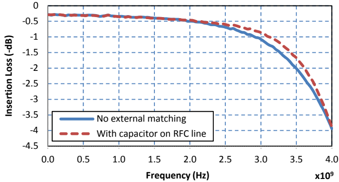
Figure 20. Insertion Loss RF1 1
