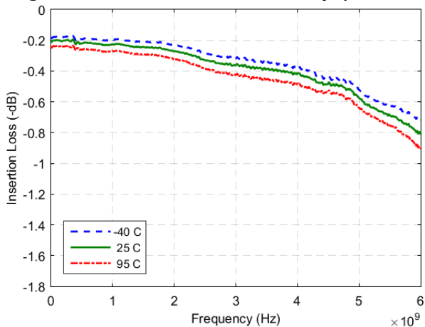
Figure 6. Insertion Loss vs Temp (RF1-RFC)*
