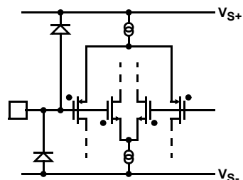
CIRCUIT 1
