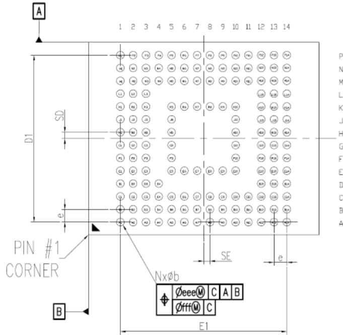
Figure 3 – Ball Pattern Dimensions
