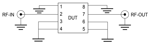
Fig 1. Block Diagram of Test Circuit used for characterization. Test Board TB-EQY-3-24+
