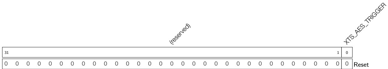
Register 21.5: XTS_AES_TRIGGER_REG (0x014C)
