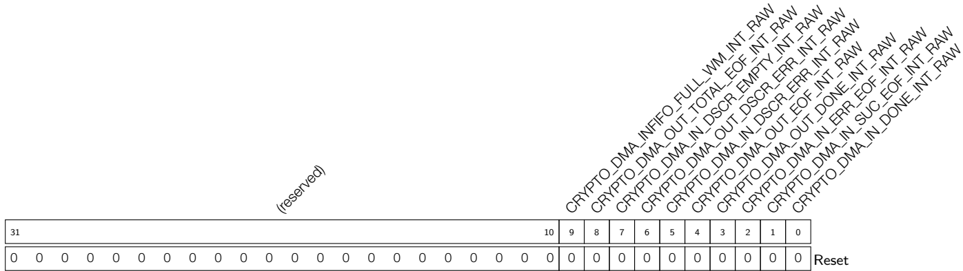
Register 2.26: CRYPTO_DMA_INT_RAW_REG (0x0004)
