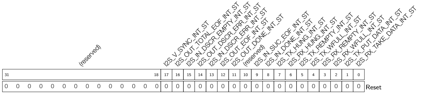
Register 26.10: I2S_INT_ST_REG (0x0010)
