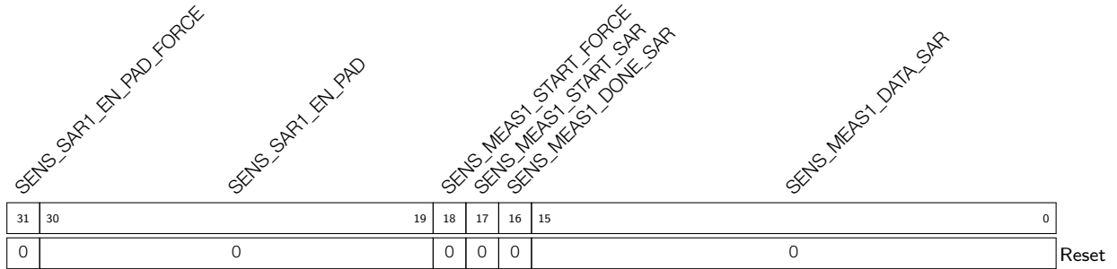
Register 32.3: SENS_SAR_MEAS1_CTRL2_REG (0x000C)
