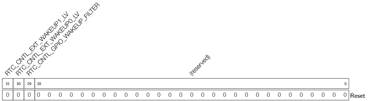
Register 9.22: RTC_CNTL_EXT_WAKEUP_CONF_REG (0x0064)
