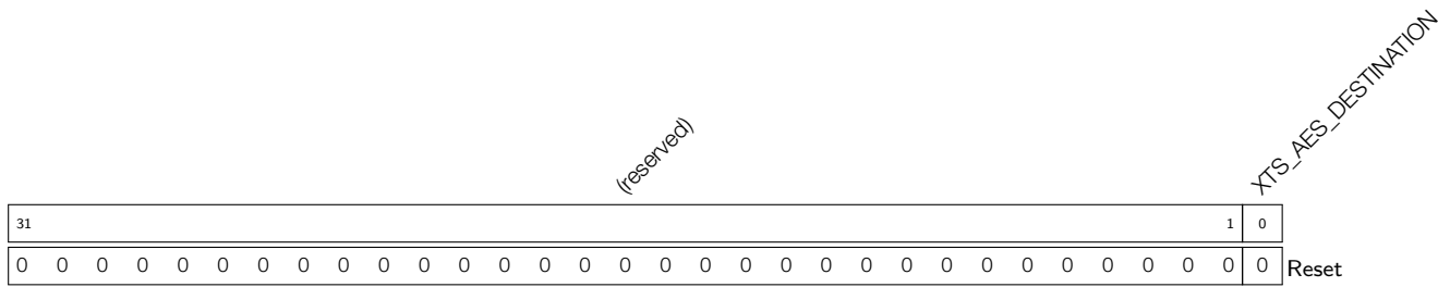
Register 21.3: XTS_AES_DESTINATION_REG (0x0144)
