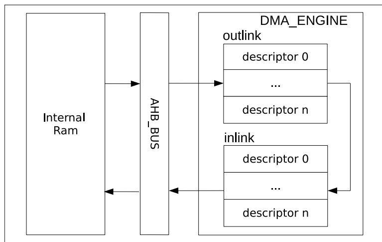
Figure 2-6. Copy DMA Engine Architecture
