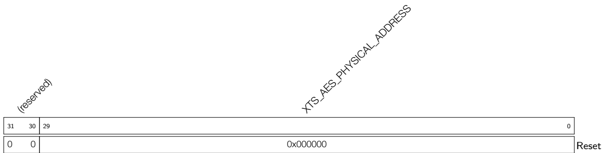
Register 21.4: XTS_AES_PHYSICAL_ADDRESS_REG (0x0148)
