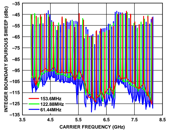
Figure 16. Integer Boundary Spurious Sweep vs. Carrier Frequency, PFD Frequencies = 61.44 MHz, 122.88 MHz, and 153.6 MHz, Loop Filter Bandwidth = 100 kHz
