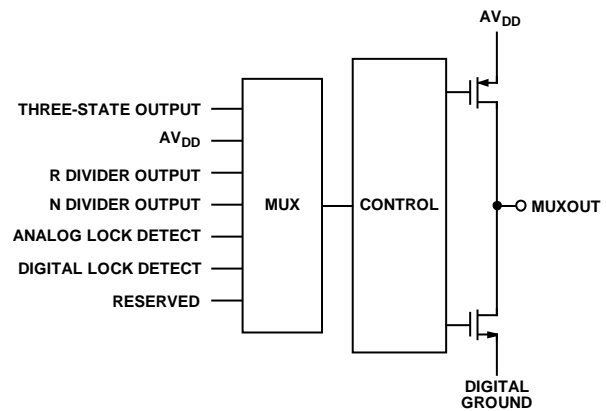
Figure 38. MUXOUT Schematic
