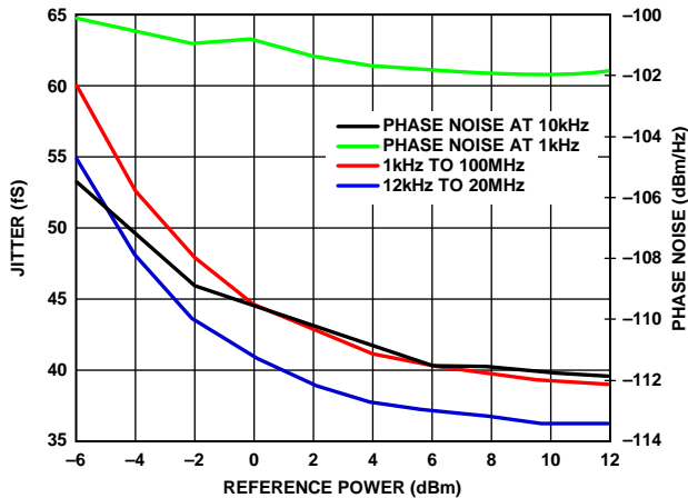
Figure 27. Jitter and Phase Noise, f_{\text{PFD}} = 250 MHz
