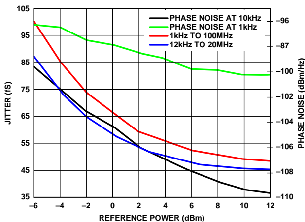
Figure 28. Jitter and Phase Noise, f_{\text{PFD}} = 100 MHz
