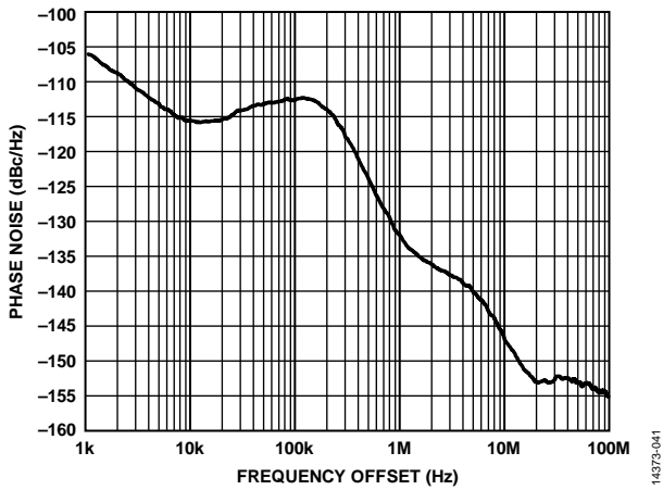
Figure 39. Phase Noise vs. Frequency Offset, RF Frequency = 460 MHz, PA2 Output Power = 17 dBm, V DD = 3.0 V, T A = 25°C
