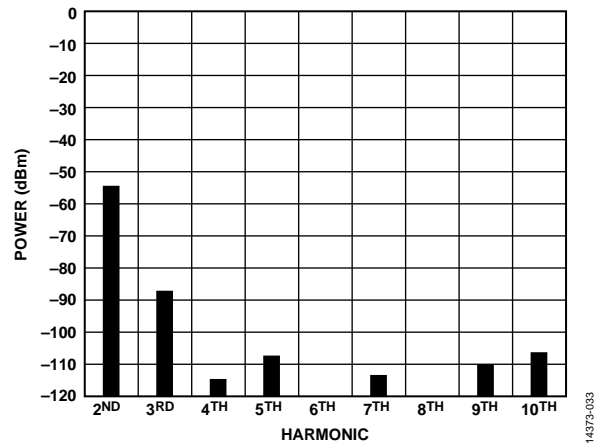
Figure 31. Conductive Harmonic Emission Level, PA1 Output Power = 10 dBm, RF Frequency = 433.92 MHz, V_{DD} = 3.0\text{ V} , T_A = 25^\circ\text{C}
