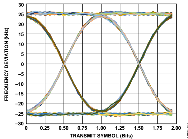
Figure 32. Transmit Eye Diagram, PA2 Output Power = 17 dBm, Configuration 433 MHz/50 kbps, V_{DD} = 3.0\text{ V} , T_A = 25^\circ\text{C}
