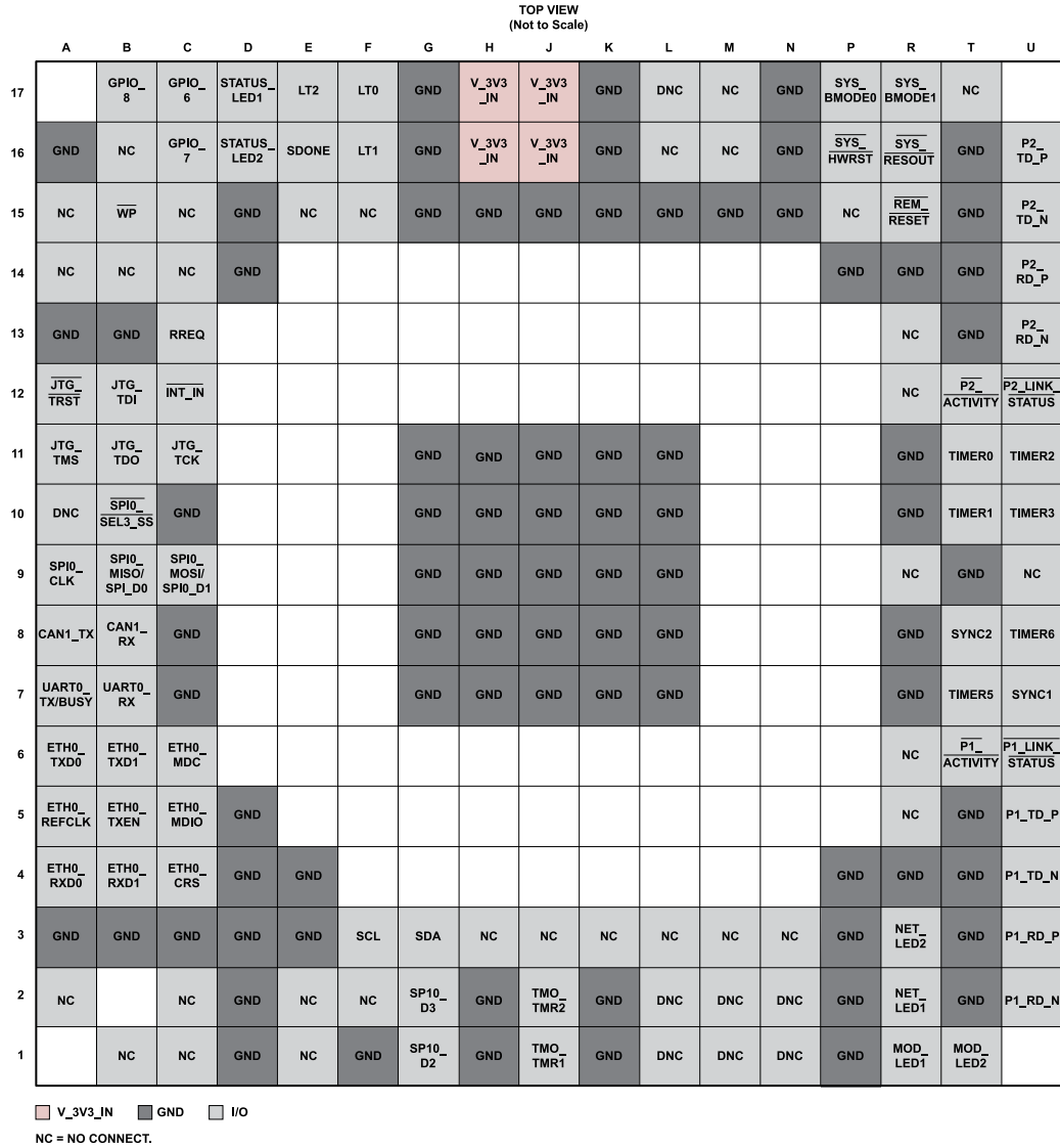
Figure 6. Ball Configuration
