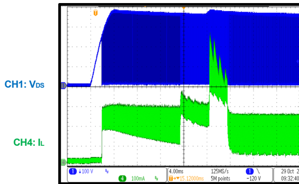
Start-Up
