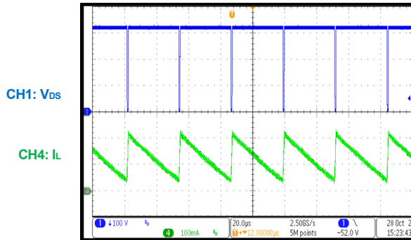
Steady State
