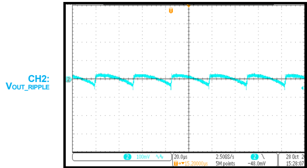
Output Ripple
