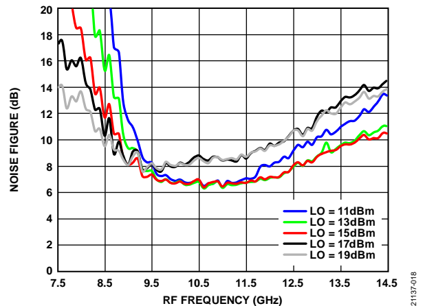
Figure 18. Noise Figure vs. RF Frequency at Various LO Power Levels, TA = 25°C
